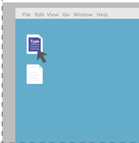
Save information
