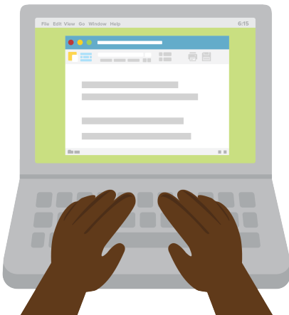
Use computer
