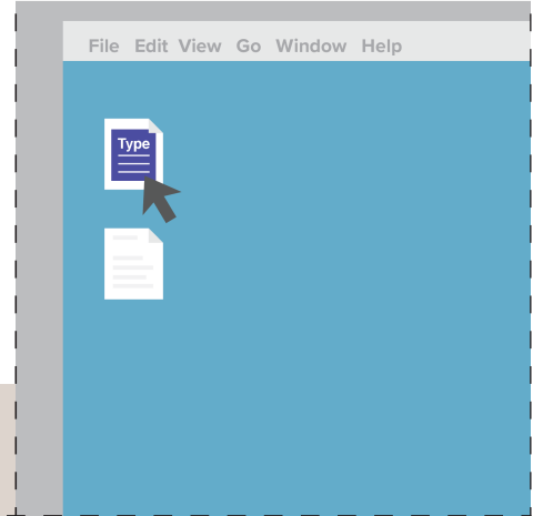
Sit down
