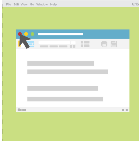
End activity
